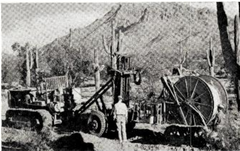
Cable plow train laying coaxial cable in difficult territory
